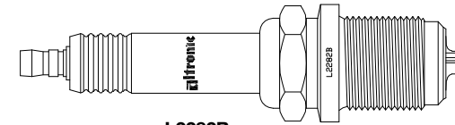
L2282B 7/8-18 SAE X 1.00" reach, Nickel CHAMPION: W77N, RW77N
