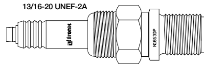
N1863DP 18mm X 1.5mm X 13/16" reach, Platinum CHAMPION: RTB77WPCC
