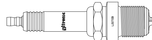
L2272B 7/8-18 SAE X .86" reach, Nickel CHAMPION: RW78N, RW83F
